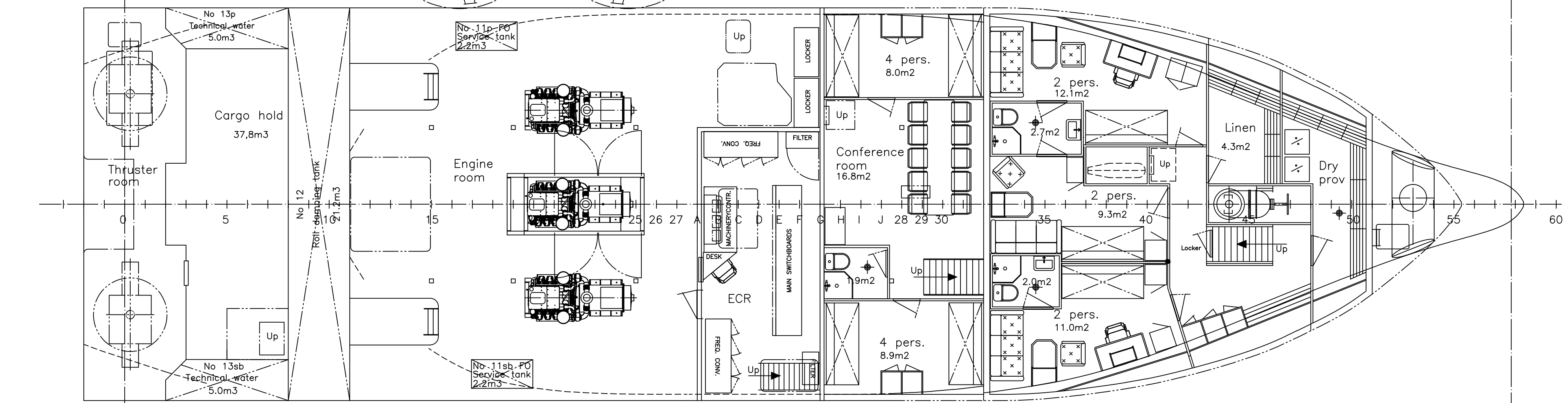
BELOW 1-DECK
