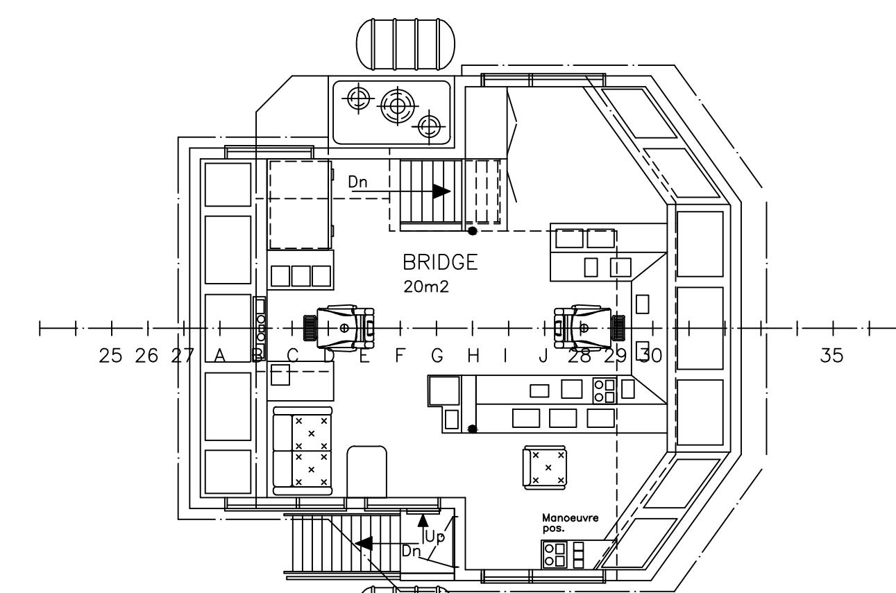
WHEEL HOUSE
